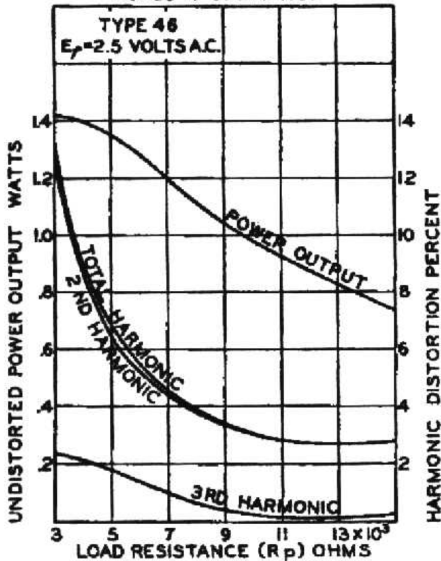
AVERAGE CHARACTERISTICS CLASS A OPERATION
