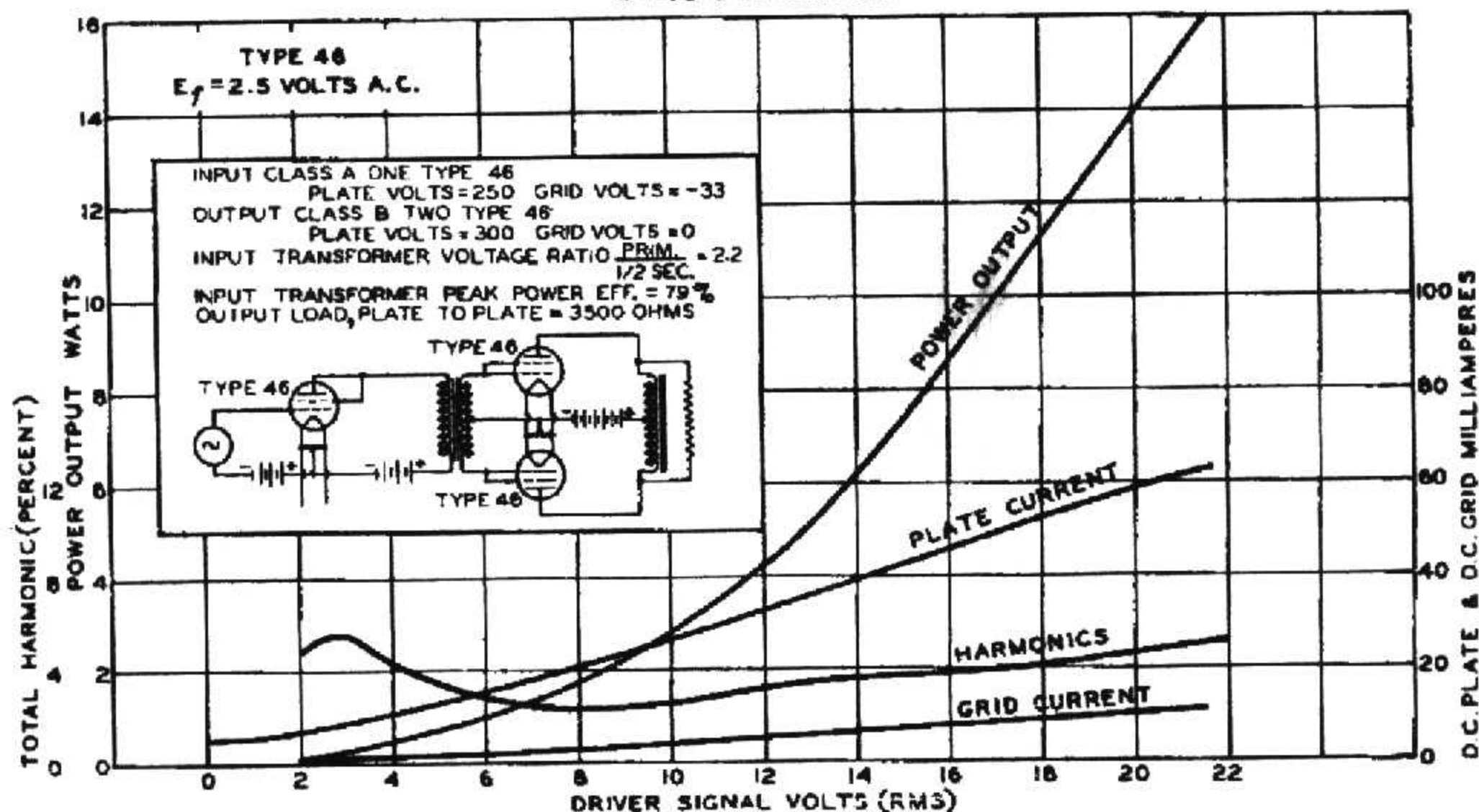
OPERATION CHARACTERISTICS CLASS B OPERATION
