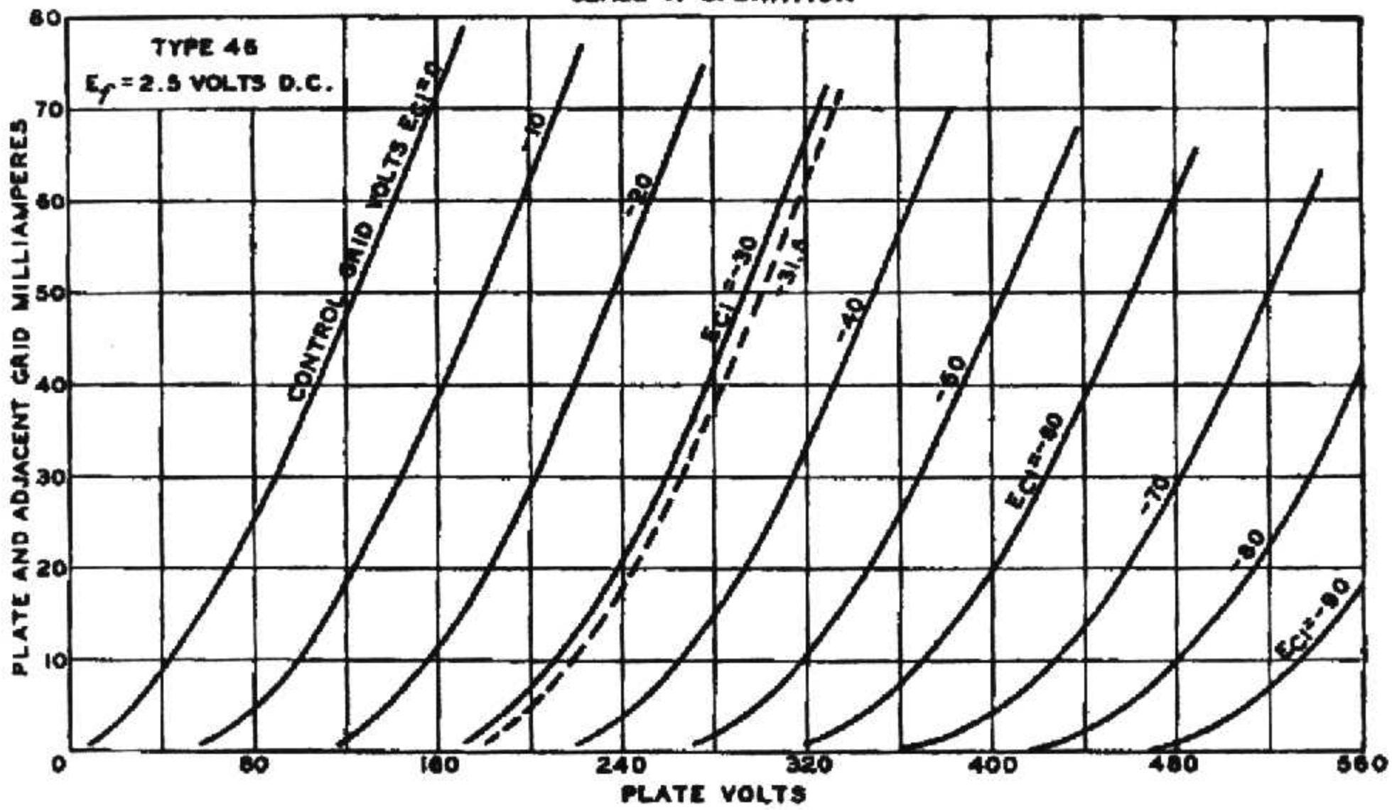
AVERAGE PLATE CHARACTERISTICS CLASS A OPERATION
