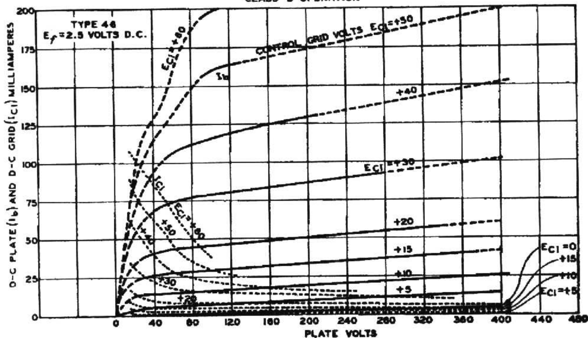
OPERATION CHARACTERISTICS CLASS B OPERATION
