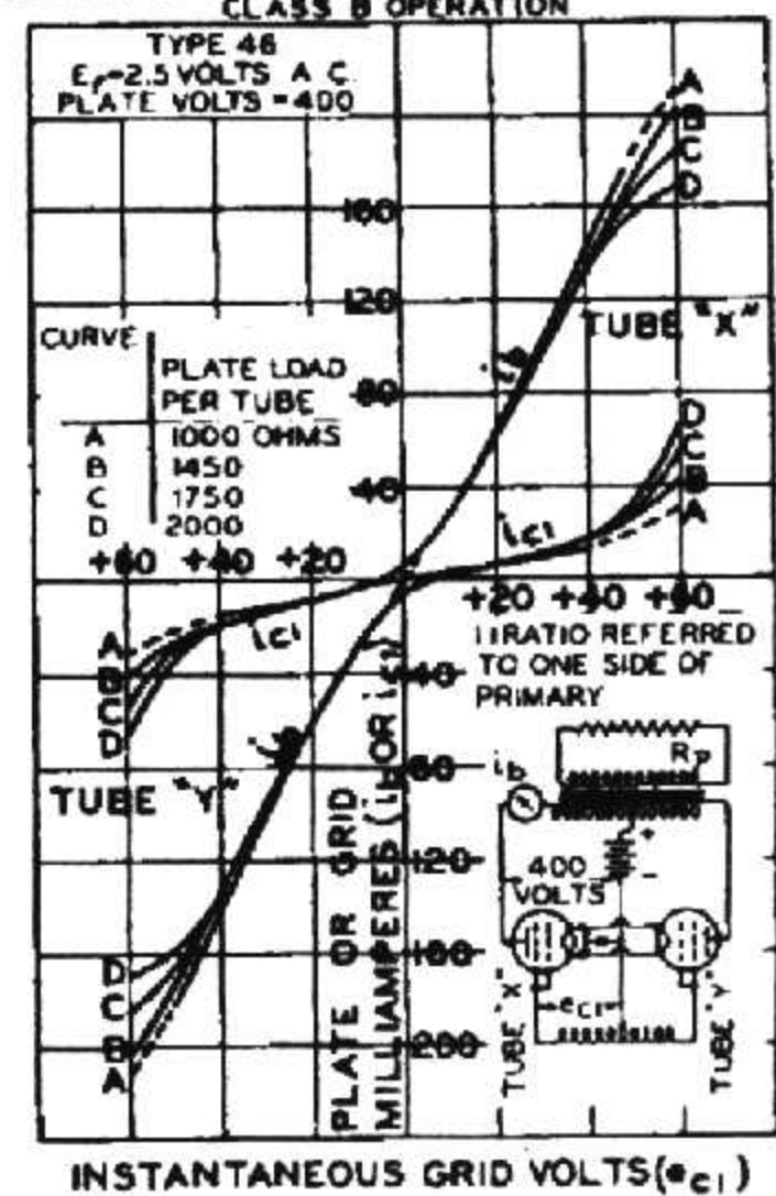
DYNAMIC TRANSFER CHARACTERISTICS CLASS B OPERATION
