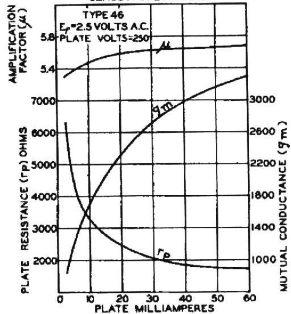
AVERAGE CHARACTERISTICS CLASS A OPERATION
